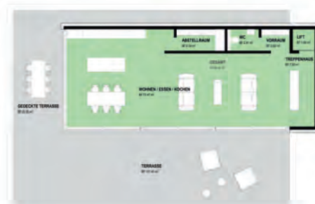
Grundriss Attikageschoss
